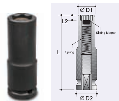
6-Point Sockets - Deep - With Slide Magnetic
