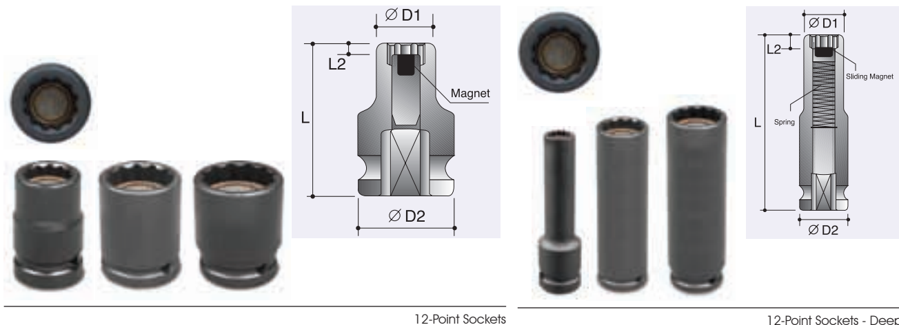
12-Point Sockets
