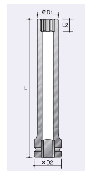
6-Point Extra Long Socket For Wheel Nuts
