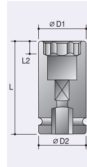
6-Point Budd Wheel Sockets - Control Depth Hex
