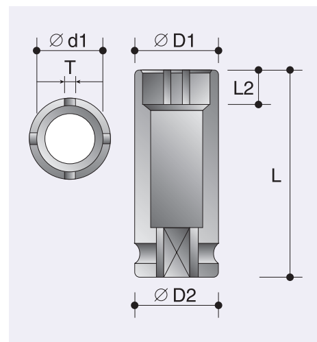
"KM" Type Axial Nut Sockets
