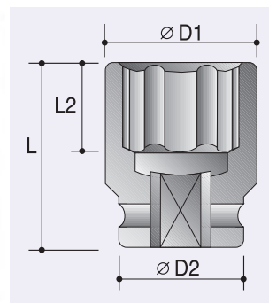
6-Point, Spindle Nut Impact Sockets
