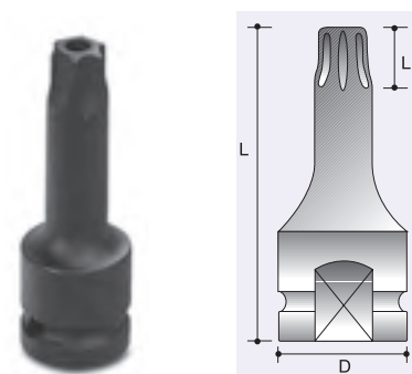
Internal Torx Drivers - With Tamper Resistant
