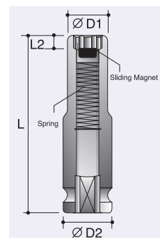
External Torx Sockets - Deep - With Slide Magnetic
