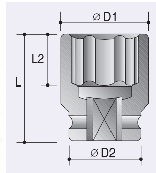
4-Point Sockets
