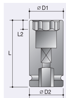
Combination Budd Wheel Sockets
