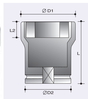
6-Point Truck Pinion Sockets
