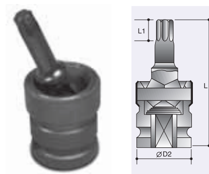
Universal Internal Torx Drivers
