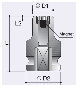
External Torx Sockets - With Magnetic
