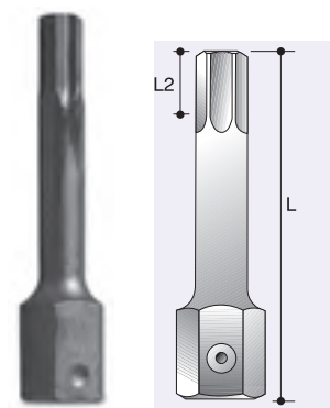
Internal Torx
